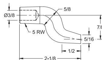
16-3871 RWMA CLASS 2 COLD FORMED*
