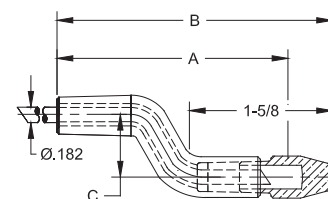
BENT OFFSET SHANKS FOR MALE CAPS WITH #4 RW TAPERS
