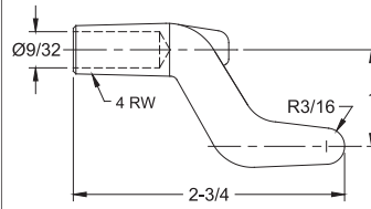
16-3837 RWMA CLASS 2 CASTING
