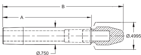
SHANKS FOR MALE CAPS WITH #6 RW TAPERS
