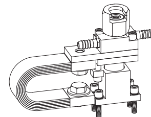
18-826 Complete #1 size "NU-TWIST"® Hydraulic assembly see page 54 for 5RW cap electrode, 4 RW, & 5 RW electrode complete #1 size assemblies
