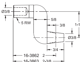
16-3862 2 16-3863 2-3/8 RWMA CLASS 2 FORGED
