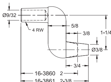
16-3860 2 16-3861 2-3/8 RWMA CLASS 2 FORGED
